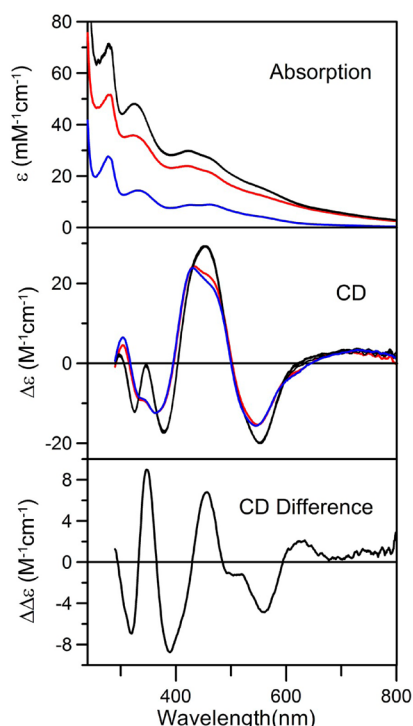
Figure 9. Time course of cluster transfer from [4\text{Fe-4S}]^{2+} cluster-bound NifU to apo- \text{NifIscA} monitored by UV–visible absorption and CD spectroscopies under anaerobic conditions at room temperature in the absence of DTT. Upper and middle panels show UV–visible absorption and CD spectra of the reaction mixture containing [4\text{Fe-4S}]^{2+} cluster-bound NifU ( 35\ \mu\text{M} in NifU monomer with one [4\text{Fe-4S}]^{2+} clusters and one permanent [2\text{Fe-2S}]^{2+} cluster per monomer) and apo- \text{NifIscA} ( 100\ \mu\text{M} in \text{NifIscA} dimer) recorded before addition of apo- \text{NifIscA} (zero time, red lines) and 5, 10, 20, 30, and 50 min after addition of apo- \text{NifIscA} (overlapping black lines). The UV–visible absorption and CD spectra of NifU containing only the permanent [2\text{Fe-2S}]^{2+} cluster are shown for comparison (blue lines). The lower panel shows the 50 min minus zero time difference CD spectrum that is characteristic of [2\text{Fe-2S}]^{2+} cluster-bound \text{NifIscA} . All \epsilon , \Delta\epsilon , and \Delta\Delta\epsilon values are expressed per NifU monomer.
