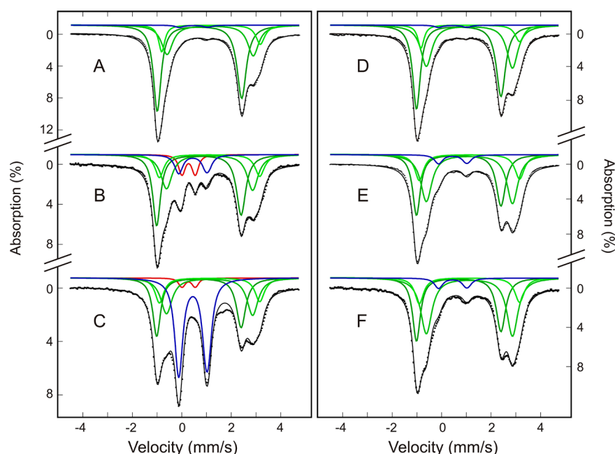
Figure 2. Time-dependent Mössbauer spectra of NifS-mediated Fe–S cluster assembly on NifIscA. The reconstitution mixture with (left panel) and without (right panel) NifIscA was frozen at time intervals of 2 min (A and D), 20 min (B and E), and 60 min (C and F). See Experimental Procedures for protein and reagent concentrations. The Mössbauer spectra (dotted lines) were recorded at 4.2 K in a magnetic field of 50 mT applied parallel to the \gamma -beam. The colored lines are theoretical simulations for the individual Fe species using the parameters listed in Table 1: Fe II Cys 4 , Fe II -3.5, and Fe II -4.1 in green; [2Fe-2S] 2+ cluster in red; [4Fe-4S] 2+ cluster in blue. They are plotted in accord with the percentage absorptions listed in Table 2. The solid black lines overlaid with the experimental spectra are composites of the simulations shown.
