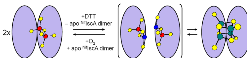
Figure 10. Proposed mechanism for [2\text{Fe-2S}]^{2+} and [4\text{Fe-4S}]^{2+} cluster interconversion on \text{NifIscA} (red, \text{Fe}^{3+} ; blue \text{Fe}^{2+} ; green, \text{Fe}^{2.5+} ; yellow, S).
