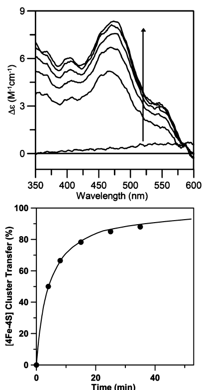
Figure 8. Time course of cluster transfer from [4\text{Fe-4S}]^{2+} cluster-bound \text{NifIscA} to A. vinelandii apo ADP-bound nitrogenase Fe protein monitored by UV–visible CD spectroscopy under anaerobic conditions. Top panel: CD spectra of apo ADP-bound nitrogenase Fe protein ( 12.5\ \mu\text{M} in dimer in final reaction mixture) were recorded before (zero time) and after reaction with [4\text{Fe-4S}]^{2+} cluster-bound \text{NifIscA} ( 12.5\ \mu\text{M} in [4\text{Fe-4S}]^{2+} clusters in the final reaction mixture) for 4, 8, 15, 25, and 35 min. The arrow indicates an increase in CD intensity with increasing time. \Delta\epsilon values are based on the initial \text{NifIscA} [4\text{Fe-4S}]^{2+} cluster concentration. Bottom panel: Kinetics of [4\text{Fe-4S}]^{2+} cluster based on CD intensity of holo ADP-bound nitrogenase Fe protein at 475 nm as function of time. The solid line is the best fit kinetic simulation for direct cluster transfer with a second order rate constant of 20\,000\ \text{M}^{-1}\ \text{min}^{-1} .
