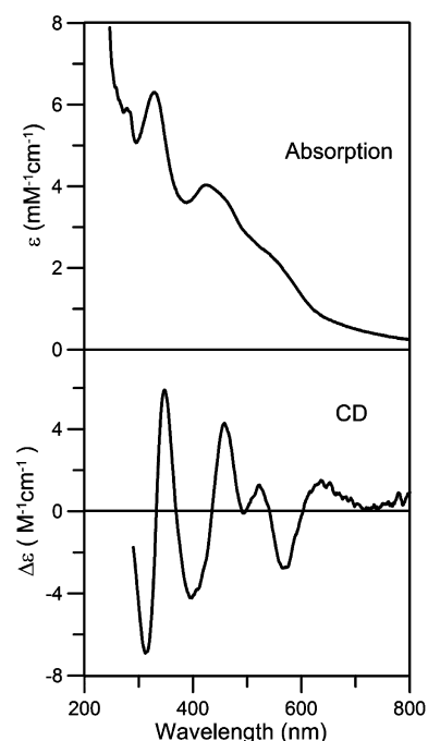
Figure 3. UV–visible absorption and visible CD spectra of the purified [2\text{Fe-2S}]^{2+} cluster-bound form of \text{Nif}^{\text{IscA}} recorded at room temperature under anaerobic conditions in septum-sealed 1 mm quartz cuvettes. Molar extinction coefficients ( \epsilon ) values are based on the concentration of monomeric \text{Nif}^{\text{IscA}} as determined by protein assays and \Delta\epsilon values are based on the concentration of \text{Nif}^{\text{IscA}} -bound [2\text{Fe-2S}]^{2+} clusters.
