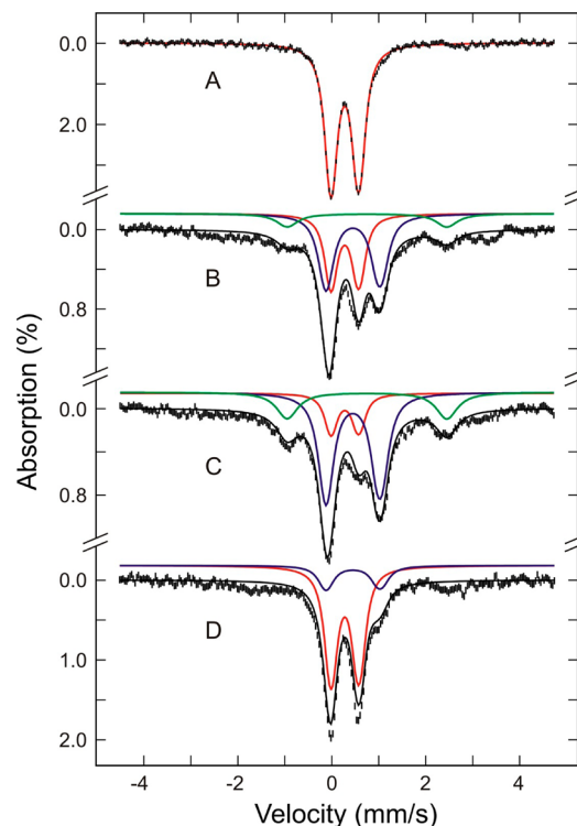
Figure 5. DTT-induced [2\text{Fe-2S}]^{2+} -to- [4\text{Fe-4S}]^{2+} cluster conversion and \text{O}_2 -induced [4\text{Fe-4S}]^{2+} -to- [2\text{Fe-2S}]^{2+} cluster conversion on \text{NifIscA} monitored by Mössbauer spectroscopy. Mössbauer spectra (hashed marks) were recorded at 4.2 K in a magnetic field of 50 mT applied parallel to the \gamma -beam. The spectra shown are for reconstituted and repurified [2\text{Fe-2S}]^{2+} cluster-bound \text{NifIscA} (0.5 mM in [2\text{Fe-2S}]^{2+} clusters) prior to addition of 2.0 mM DTT (A), 1 min after DTT addition (B), 15 min after DTT addition (C), and after exposing the 15 min DTT-treated sample to air for 5 min (D). The colored lines are theoretical simulations for the individual Fe species (Fe(II) species in green, [2\text{Fe-2S}]^{2+} clusters in red and [4\text{Fe-4S}]^{2+} clusters in blue) using the parameters listed in Table 1 and plotted in percentages listed in Table 4. The solid black lines overlaid with the experimental spectra are the composite spectra.
