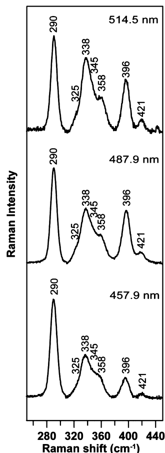
Figure 4. Resonance Raman spectra of purified [2\text{Fe-2S}]^{2+} -bound form of \text{NifIscA} . Raman spectra were recorded at 17 K with 457.9, 487.9, and 514.5 nm laser excitation with \sim 185 mW laser power at the sample. The sample ( \sim 2 mM in [2\text{Fe-2S}]^{2+} clusters) was in 100 mM Tris-HCl buffer, pH 7.8 containing \sim 0.45 M NaCl. Each spectrum is a sum of 100 scans, with each scan involving counting photons for 1 s at 0.5\text{ cm}^{-1} increments with 6\text{ cm}^{-1} spectral resolution. Bands due to lattice modes of ice from frozen buffer in sample have been subtracted from all spectra.
