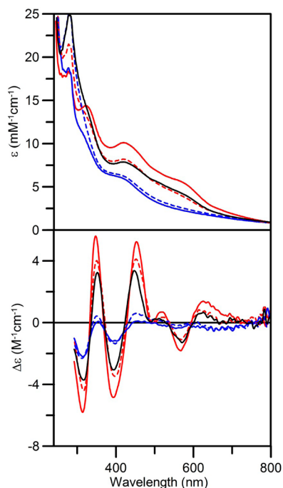
Figure 6. [2\text{Fe-}2\text{S}]^{2+} \leftrightarrow [4\text{Fe-}4\text{S}]^{2+} cluster interconversions on \text{Nif}^{\text{IscA}} monitored by UV–visible absorption and CD spectroscopies. Anaerobically purified [2\text{Fe-}2\text{S}]^{2+} cluster-bound (solid red line) was treated with 2 mM DTT and incubated for 15 min (solid blue line), exposed to air for 5 min (broken red line), sealed and incubated for an additional 15 min (broken blue line), and exposed to air again for 5 min (solid black line). \epsilon and \Delta\epsilon values are based on the [2\text{Fe-}2\text{S}]^{2+} cluster concentration of the initial [2\text{Fe-}2\text{S}]^{2+} cluster-bound \text{Nif}^{\text{IscA}} sample (0.05 mM). The CD spectra of the first and second air-exposed samples have been corrected for contributions from \text{Fe(III)-bound Nif}^{\text{IscA}} , by subtracting CD spectra of \text{Fe(III)-bound Nif}^{\text{IscA}} (see accompanying manuscript) corresponding to 10% and 20% of the total Fe, respectively.
