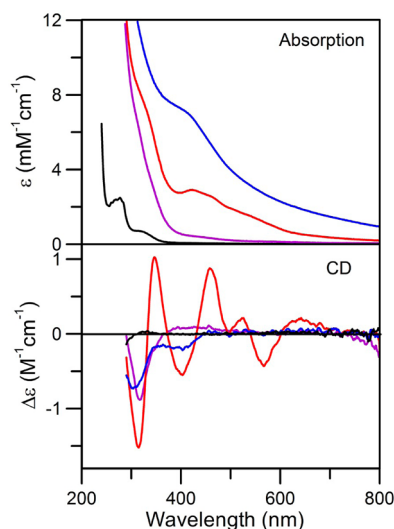
Figure 1. NifS-mediated Fe–S cluster assembly on \text{Nif}^{\text{IscA}} monitored as a function of time by UV–visible absorption and CD spectroscopies. Protein and reagent concentrations are described in the Materials and Methods. The spectra shown are for TCEP pretreated apo- \text{Nif}^{\text{IscA}} before reconstitution (black) and after 5 min (purple), 20 min (red), and 65 min (blue) of NifS-mediated Fe–S cluster assembly. \epsilon and \Delta\epsilon values are expressed per \text{Nif}^{\text{IscA}} monomer.
